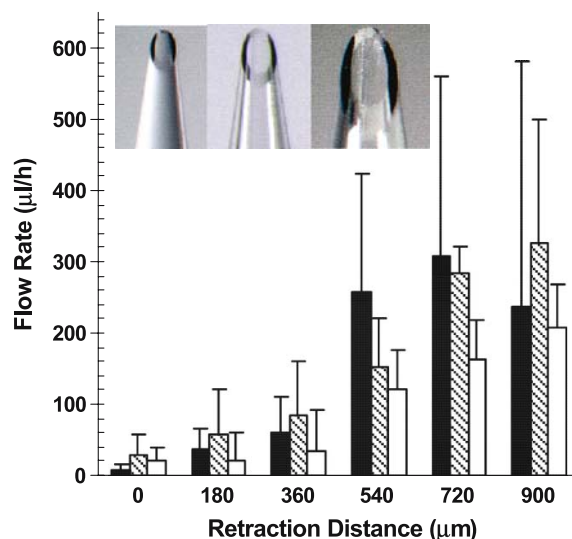
Fig. 7. Effect of tip opening size on flow rate into human cadaver skin. Microinfusion flow rate was measured as a function of retraction distance using three different tip opening sizes: 22 µm (black bars; left inset image), 30 µm (striped bars; center inset image), and 48 µm (white bars; right inset image) effective radii. Microneedles having 35–37° beveled tips were inserted to a maximum depth of 1080 µm, and infusion was carried out at 138 kPa. Data are expressed as mean values ( n \geq 3 ) with standard deviation bars.
